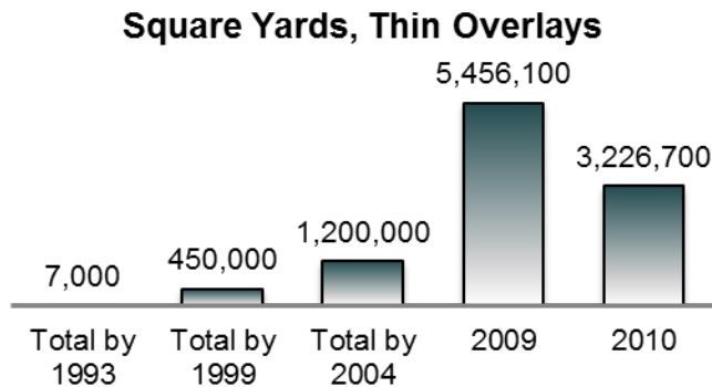
Figure 1. Construction totals of thin (<6 inches) concrete overlays in the United States.
